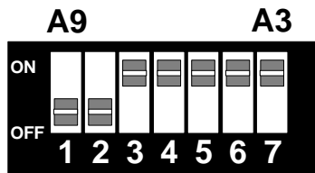
Figure 2 - DIP-switch Illustration
