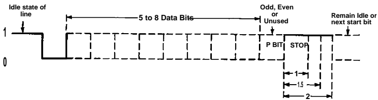
Figure 10 - Asynchronous Communications Bit Diagram
